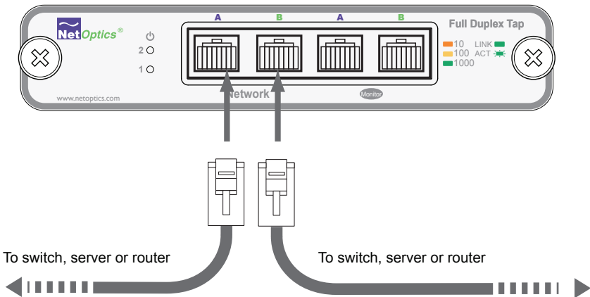
Figure 5: Connecting to the Network
