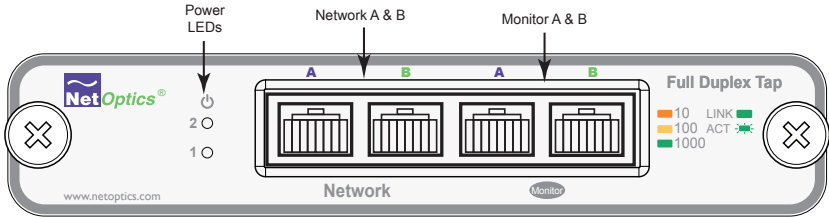
Figure 2: Front Panel, 10/100/1000BaseT Taps (TP-CU3, TP-CU3-DC)
