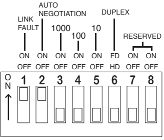
NOTE: To activate, push buttons UP. (This diagram shows all seams)
