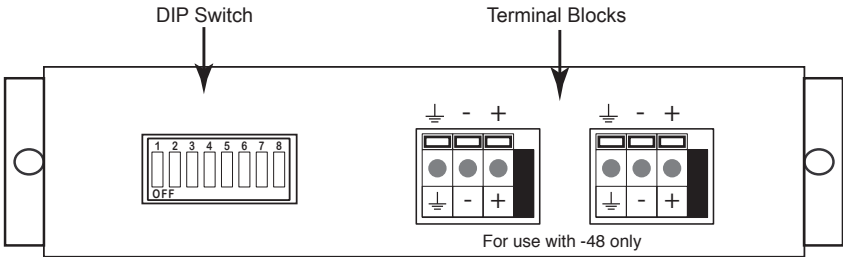
Figure 4: Rear Panel DC power models
