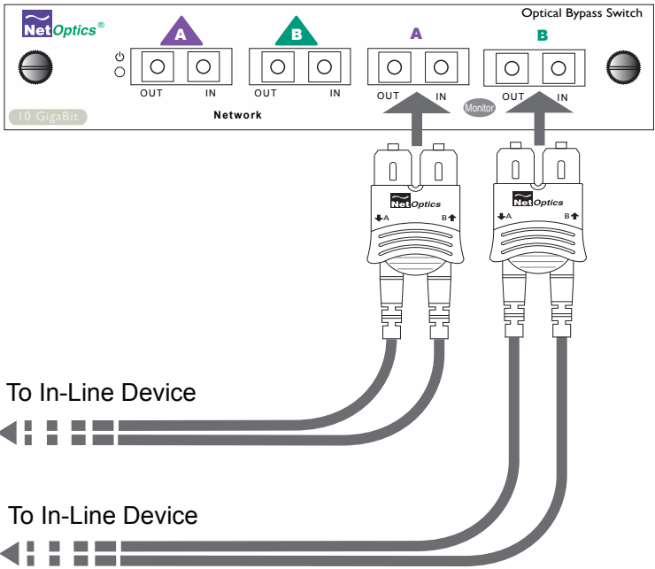
Figure 7: Connecting to the In-line Device
