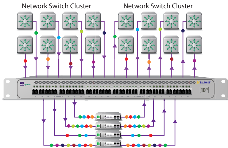
Inline load balancing of eight independent links
