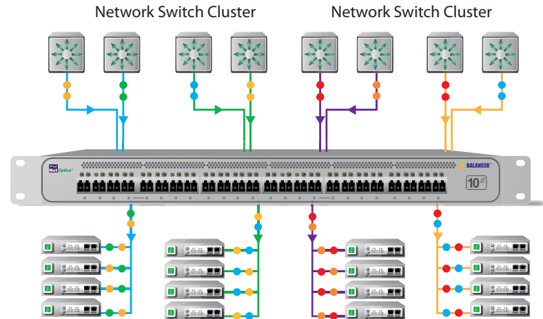
Four independent out-of-band load balancers
