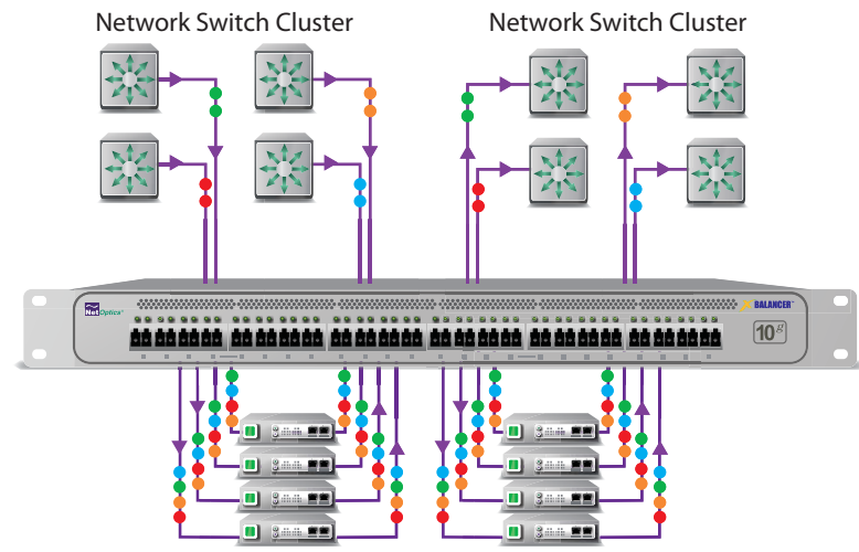
Four links to eight inline tools
